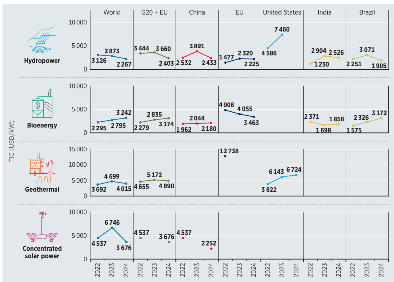
Figure 1.7 TIC trajectories of dispatchable technologies in selected regions, 2022-2024
