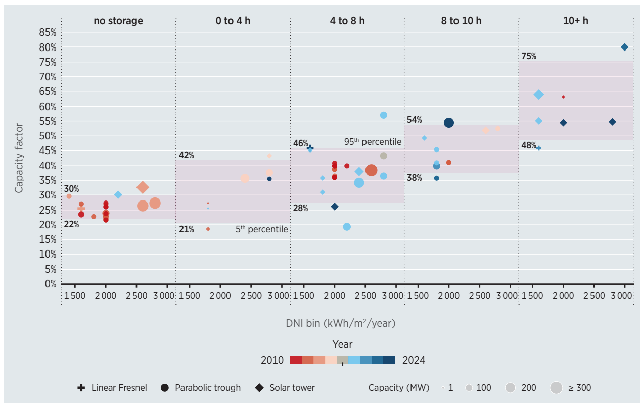
Figure 5.3 Capacity factor trends for CSP plants by DNI and storage duration, 2010–2024
