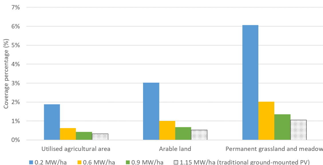
Figure 2. Required percentage of different land coverage for Agri-PV systems for the accomplishment of the EU total New Policy Trends NECP PV 2030 target for different assumed installed capacities.
