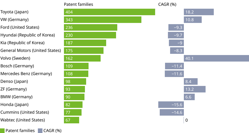
Figure 6.5 Top patent owners in green digitalization for heavy-duty road transport, by number of published patent families, 2000–2024, and annual patent publication growth rate, 2019–2024
